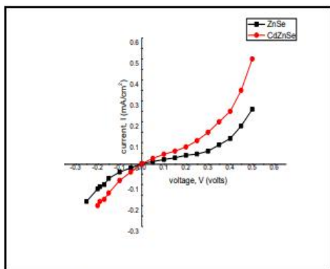
Fig.5 I- V Characteristics in dark
