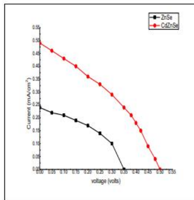
Fig.7 Power output curves
