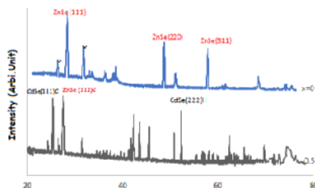
Fig.1 XRD spectra of ZnSe, Cd 0.5 Zn 0.5 Se thin films
